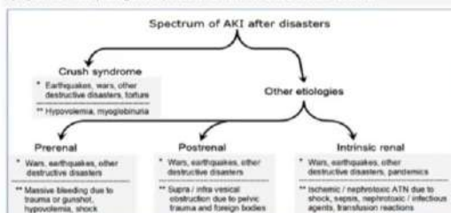
Figure 1. Spectrum of AKI after disasters. Overall, crush syndrome is very common. Similar to routine daily practice, prerenal, intrarenal or postrenal AKI may develop in various disasters, with different etio-pathogenetic mechanisms. * Most common disasters are associated with those particular pathologies. These pathologies may also be observed in several other disasters (e.g., volcanoes, mining accidents, hurricanes), albeit less frequently. ** Main pathogenetic mechanisms. (Several other mechanisms may also play a role in the pathogenesis). Abbreviation: ATN: acute tubular necrosis.
